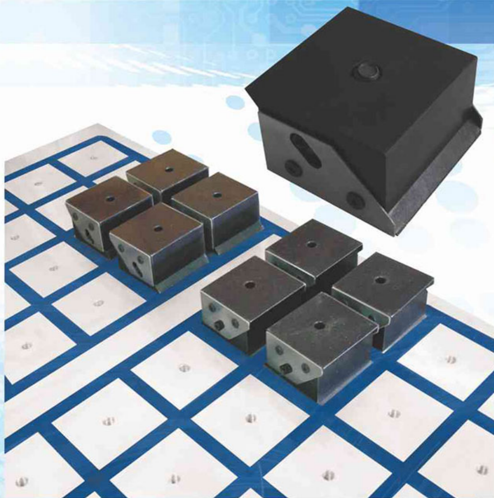
彈簧式導磁墊塊 (選購品) Spring Type Chuck Block (Optional)
